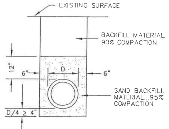
TYPE B (OUTSIDE ROADWAY)
