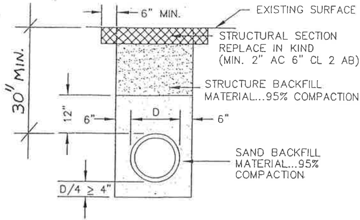
TYPE A (IN ROADWAY)
