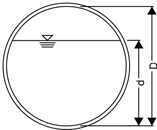
Figure 1: Proposed Flow Requirements for Connections to County Drainage Systems
