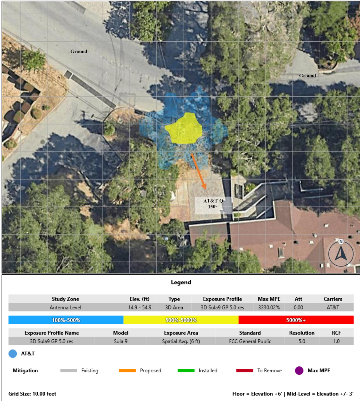
Figure1.1: Antenna Level
