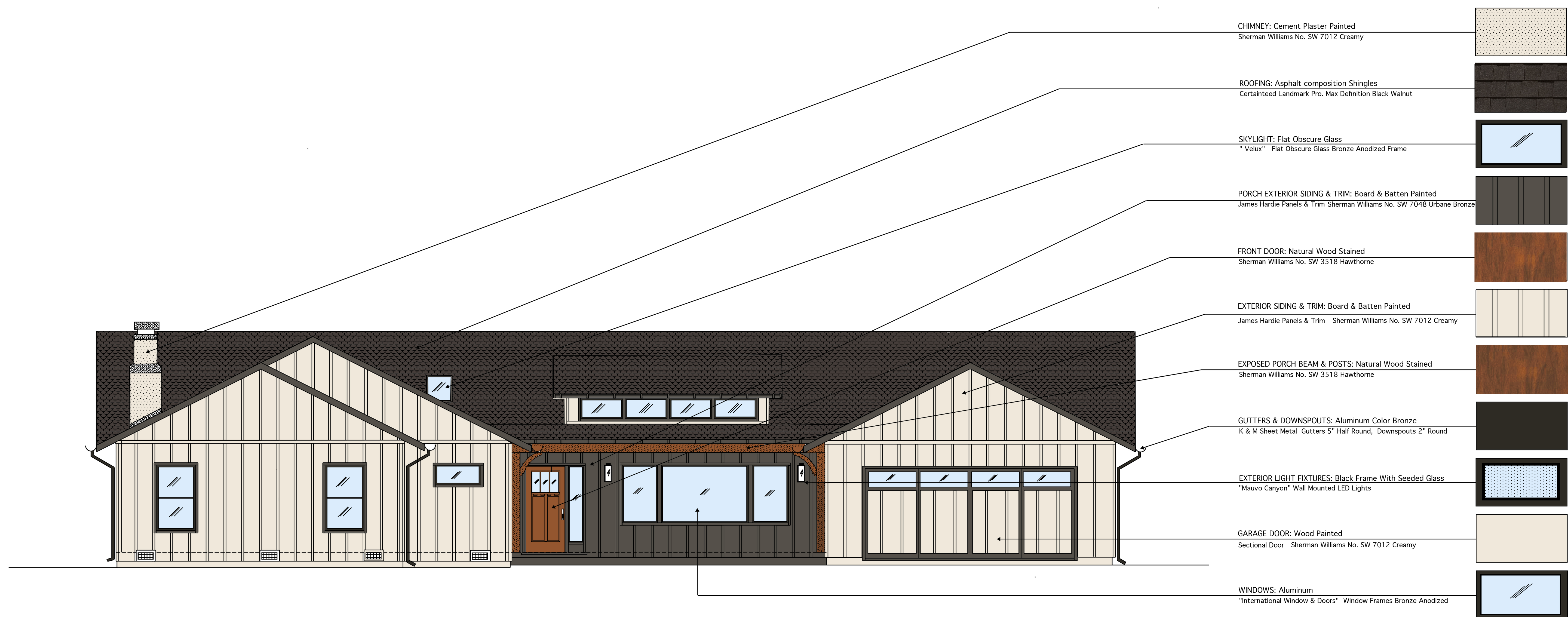
FRONT ELEVATION PROPOSED FINISHES
